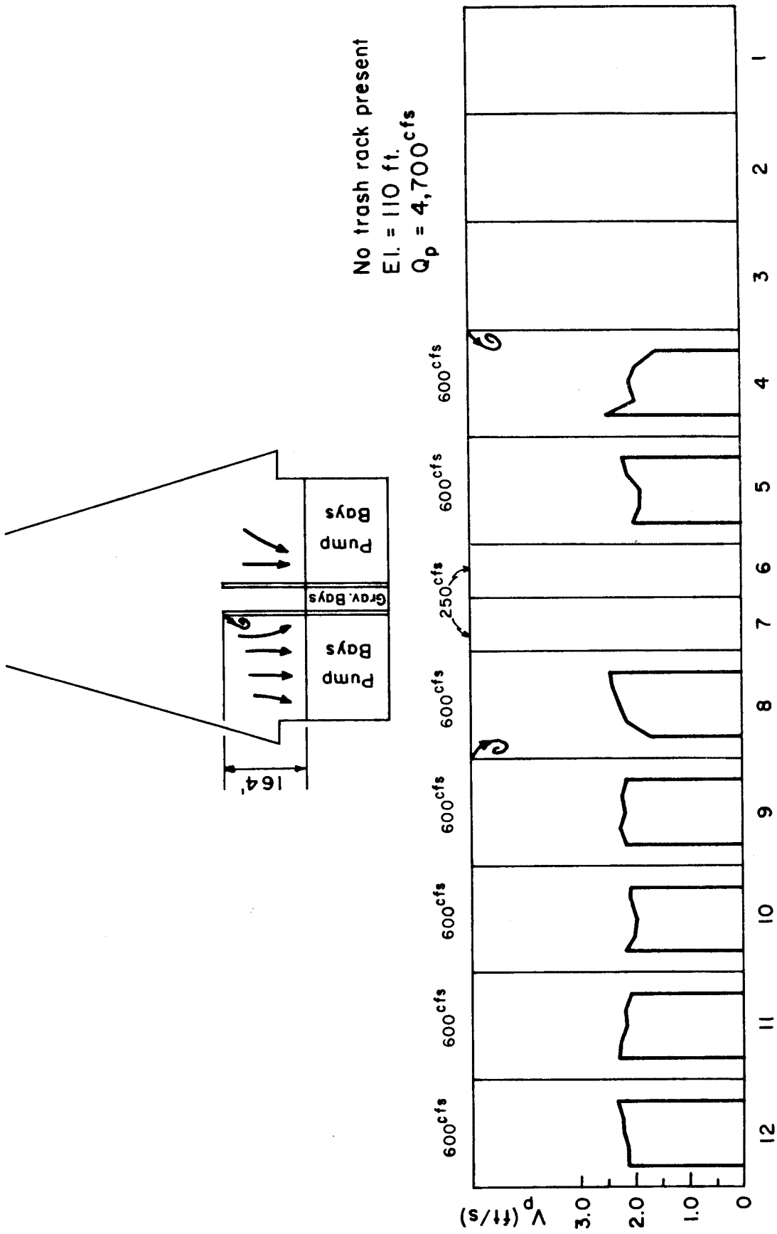
Figure 3-23. Mean velocity distributions in pump sumps (gravity-bay piers extended by 164 ft)
