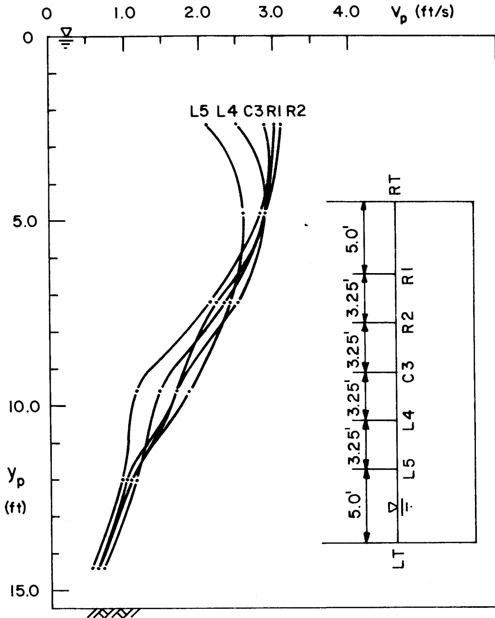
Figure 3-19. Velocity profiles obtained in Run E18' (with 9-in. deep trash rack, El. = 108.5 ft, Q_p = 600 cfs, backwall shift = 18 in., fillets = type C, splitter plate = type A')
