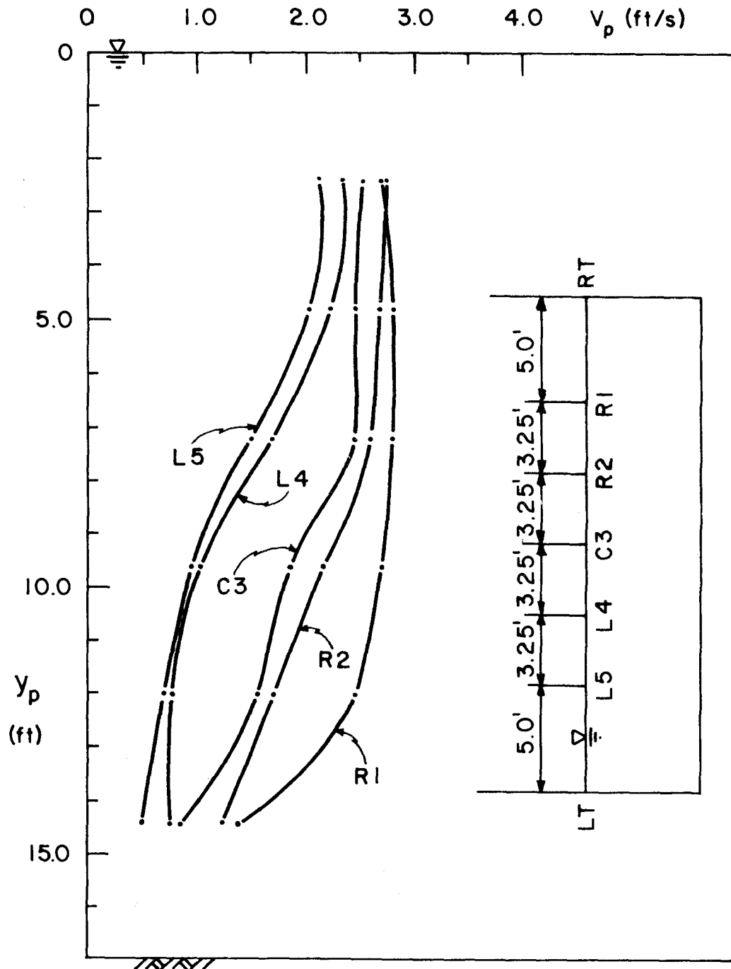
Figure 3-11. Velocity profiles obtained in Run E15' (with 12-in. deep trash rack, E1. = 110 ft, Q_p = 660 cfs, backwall shift = 18 in., fillets = type C, splitter plate = type C')
