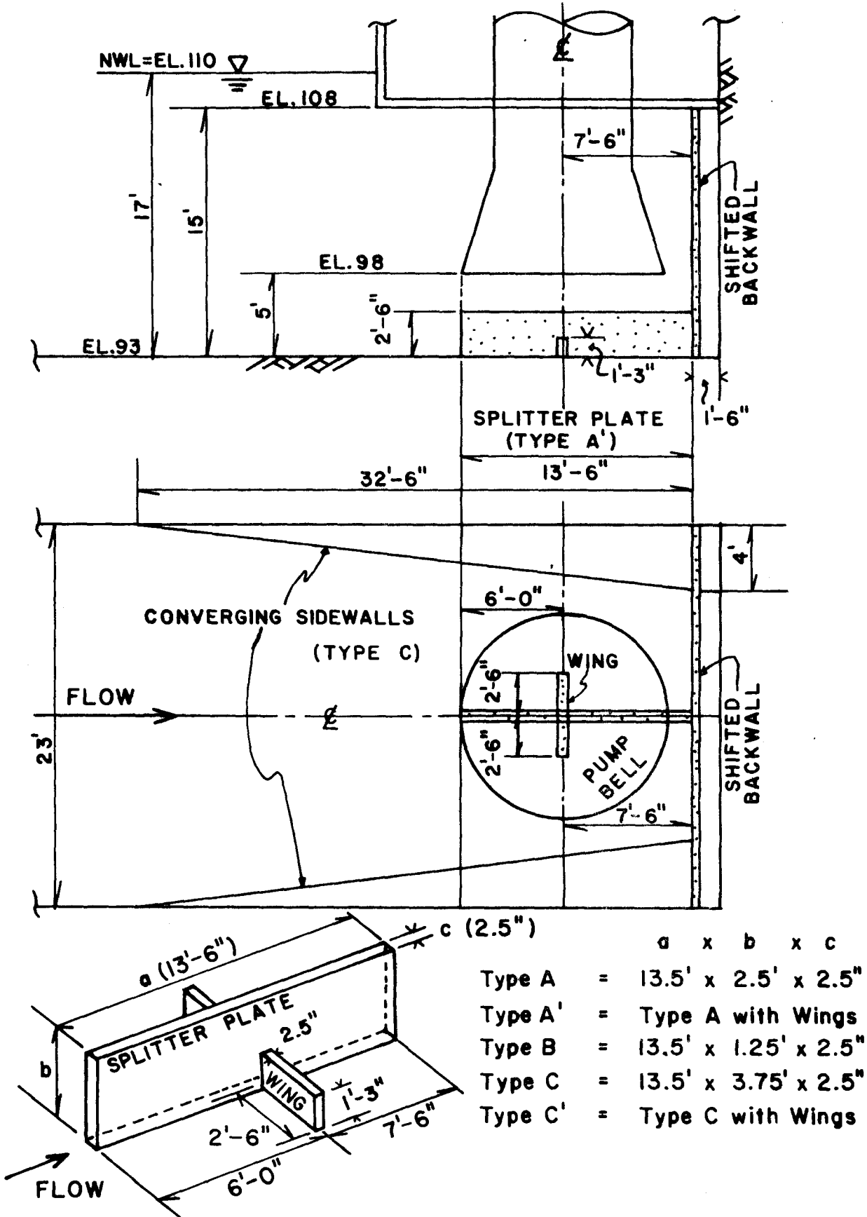
Figure 3-9. Dimensions of various splitter plates
