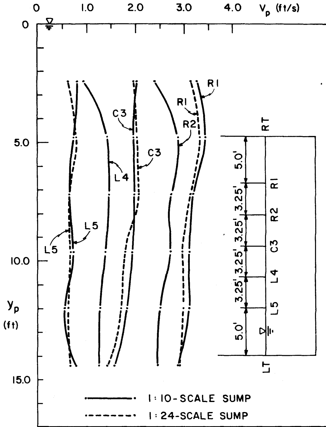
Figure 3-1. Velocity profiles obtained in both 1:10-scale and 1:24-scale models (no trash rack present, Q_p = 660 cfs, 110% operation)
