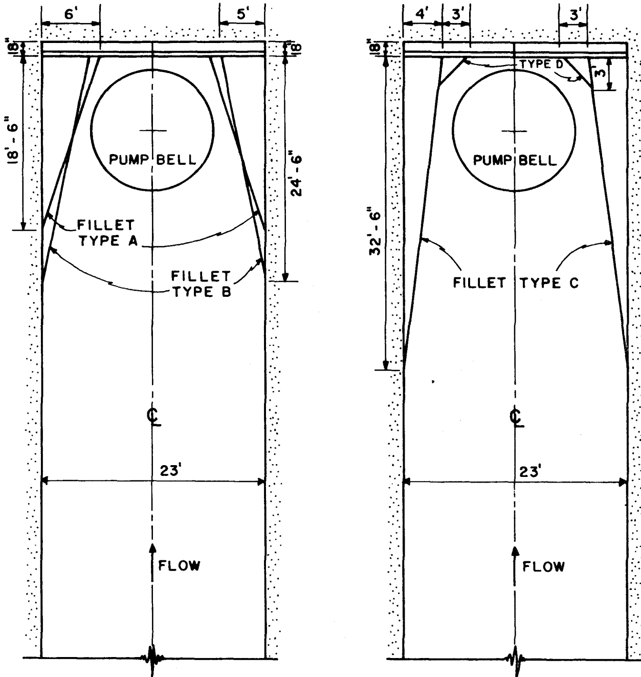
Figure 3-7. Geometrical configurations of various fillets
