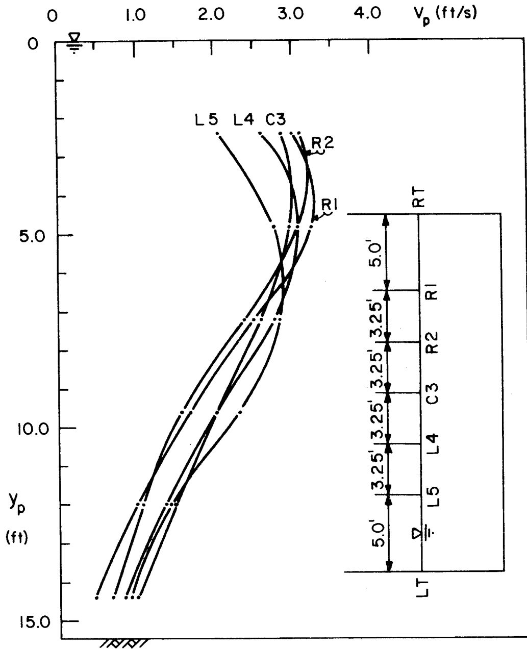
Figure 3-15. Velocity profiles obtained in Run E16' (with 9-in. deep trash rack, El. = 108.5 ft, Q_p = 660 cfs, backwall shift = 18 in., fillets = type C, splitter plate = type A')
